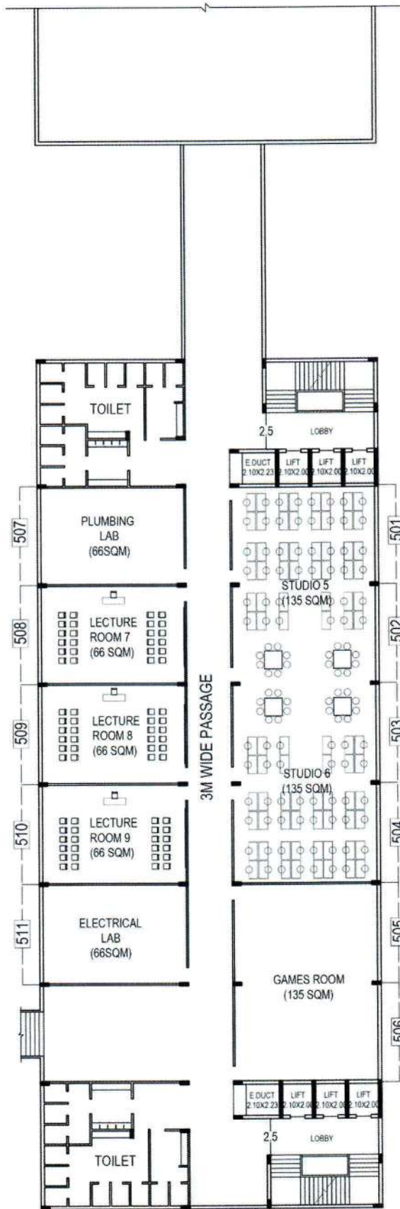
5TH FLOOR PLAN
