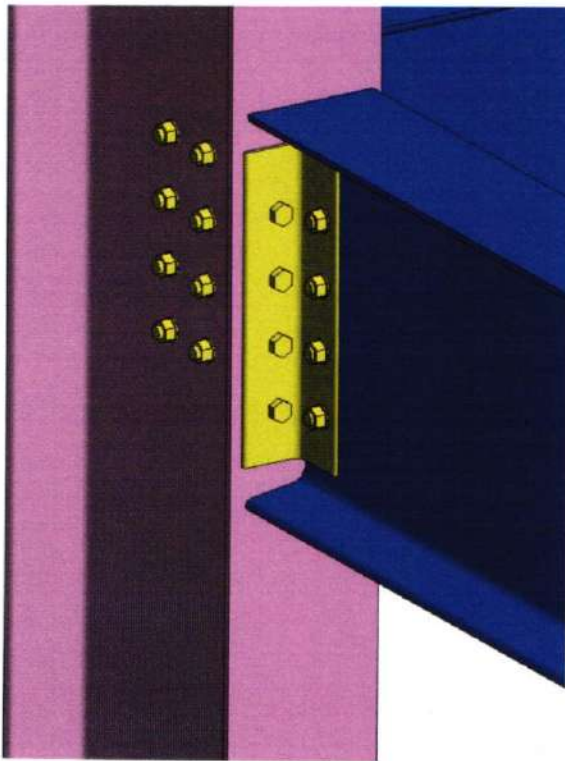
Beam to Column Flange Connection
